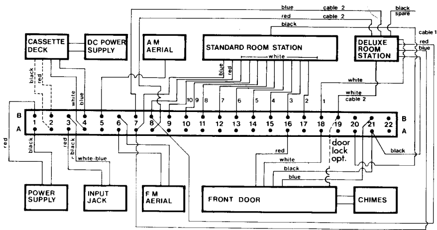
WIRING CONNECTIONS FOR GREEN EDGE CONNECTOR
